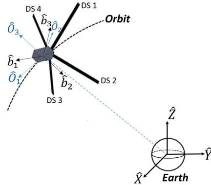
Fig. 2. Coordinate systems.
