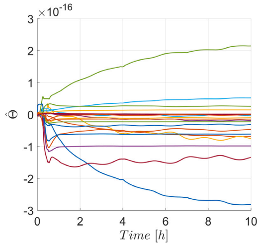
Fig. 20. Resulting parameter estimates [\hat{\epsilon}_1 \hat{B}_1 \hat{C}_{L,j}, \hat{\epsilon}_1 \hat{B}_2 \hat{C}_{L,j}, \hat{\epsilon}_2 \hat{B}_1 \hat{C}_{L,j}, \hat{\epsilon}_2 \hat{B}_2 \hat{C}_{L,j}, \hat{\epsilon}_3 \hat{B}_1 \hat{C}_{L,j}, \hat{\epsilon}_3 \hat{B}_2 \hat{C}_{L,j}]^T in \hat{\Theta} with j = 1, 2, 3, 4 associated with the aerodynamic lift for the tracking maneuver using the designed controller.
