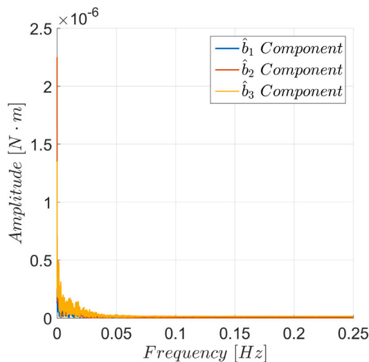
Fig. 22. FFT of the torque \hat{Y} applied during the tracking maneuver.
