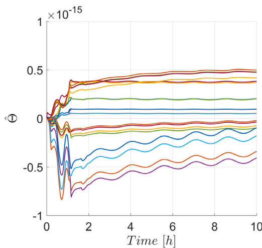
Fig. 8. Resulting parameter estimates [\hat{e}_1 \hat{B}_1 \hat{C}_{D,j}, \hat{e}_1 \hat{B}_2 \hat{C}_{D,j}, \hat{e}_2 \hat{B}_1 \hat{C}_{D,j}, \hat{e}_2 \hat{B}_2 \hat{C}_{D,j}, \hat{e}_3 \hat{B}_1 \hat{C}_{D,j}, \hat{e}_3 \hat{B}_2 \hat{C}_{D,j}]^T in \hat{\theta} with j = 1, 2, 3, 4 associated with the aerodynamic drag for the regulation maneuver using the designed controller.
