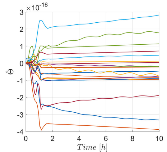
Fig. 10. Resulting parameter estimates [\hat{e}_1 \hat{B}_1 \hat{C}_{L,j}, \hat{e}_1 \hat{B}_2 \hat{C}_{L,j}, \hat{e}_2 \hat{B}_1 \hat{C}_{L,j}, \hat{e}_2 \hat{B}_2 \hat{C}_{L,j}, \hat{e}_3 \hat{B}_1 \hat{C}_{L,j}, \hat{e}_3 \hat{B}_2 \hat{C}_{L,j}]^T in \hat{\theta} with j = 1, 2, 3, 4 associated with the aerodynamic lift for the regulation maneuver using the designed controller.
