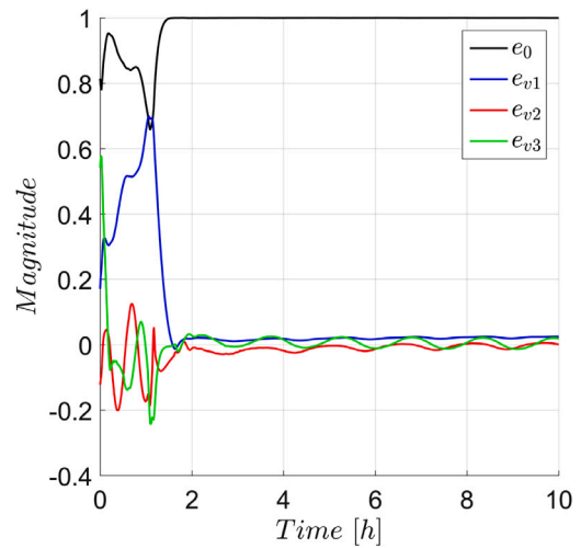
Fig. 3. Resulting error quaternion for the regulation maneuver using the designed controller.
