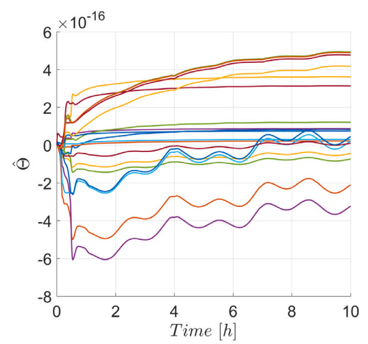
Fig. 18. Resulting parameter estimates [\hat{e}_1 \hat{B}_1 \hat{C}_{D,j}, \hat{e}_1 \hat{B}_2 \hat{C}_{D,j}, \hat{e}_2 \hat{B}_1 \hat{C}_{D,j}, \hat{e}_2 \hat{B}_2 \hat{C}_{D,j}, \hat{e}_3 \hat{B}_1 \hat{C}_{D,j}, \hat{e}_3 \hat{B}_2 \hat{C}_{D,j}]^T in \hat{\theta} with j = 1, 2, 3, 4 associated with the aerodynamic drag for the tracking maneuver using the designed controller.
